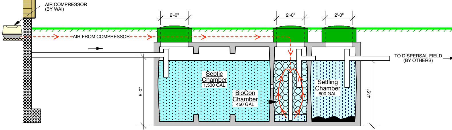
Septic/BioCon/Settling Tank 2,550 GAL 3 Compartment Tank (15'0"L x 6'6"W x 6'1"H)
