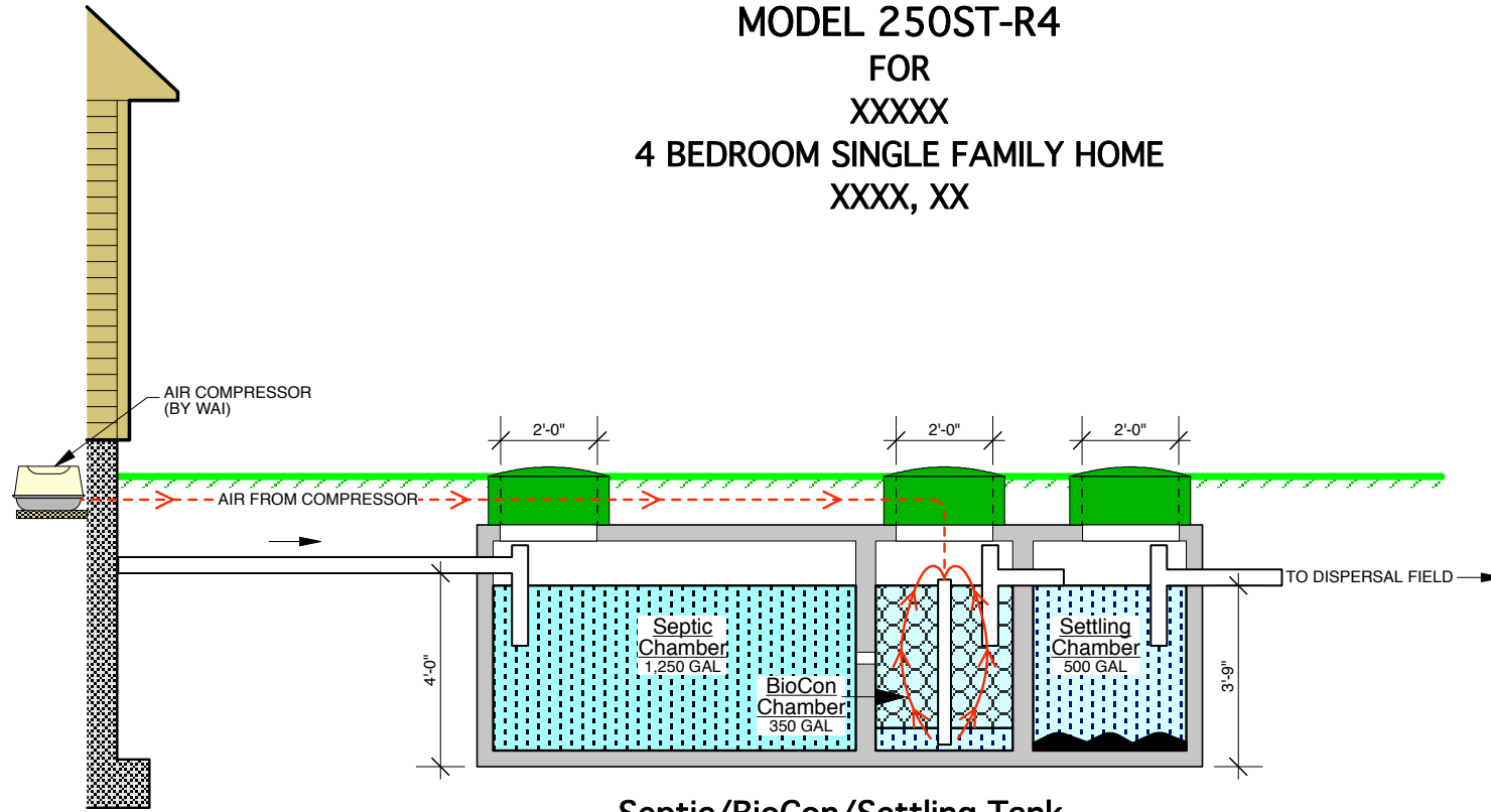
Septic/BioCon/Settling Tank 2,100 GAL 3 Compartment Tank (15'0"L x 6'6"W x 5'0"H)
