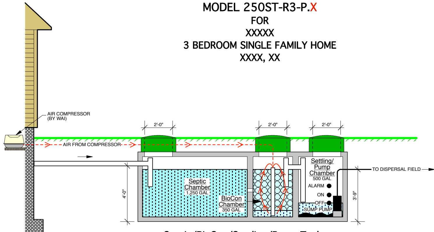
Septic/BioCon/Settling/Pump Tank 2,100 GAL 3 Compartment Tank (15'0"L x 6'6"W x 5'0"H)
