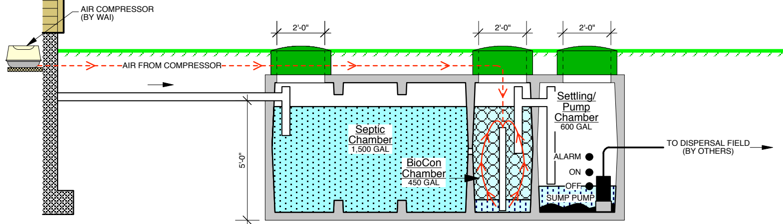
Septic/BioCon/Settling/Pump Tank 2,550 GAL 3 Compartment Tank (15'0"L x 6'6"W x 6'1"H)
