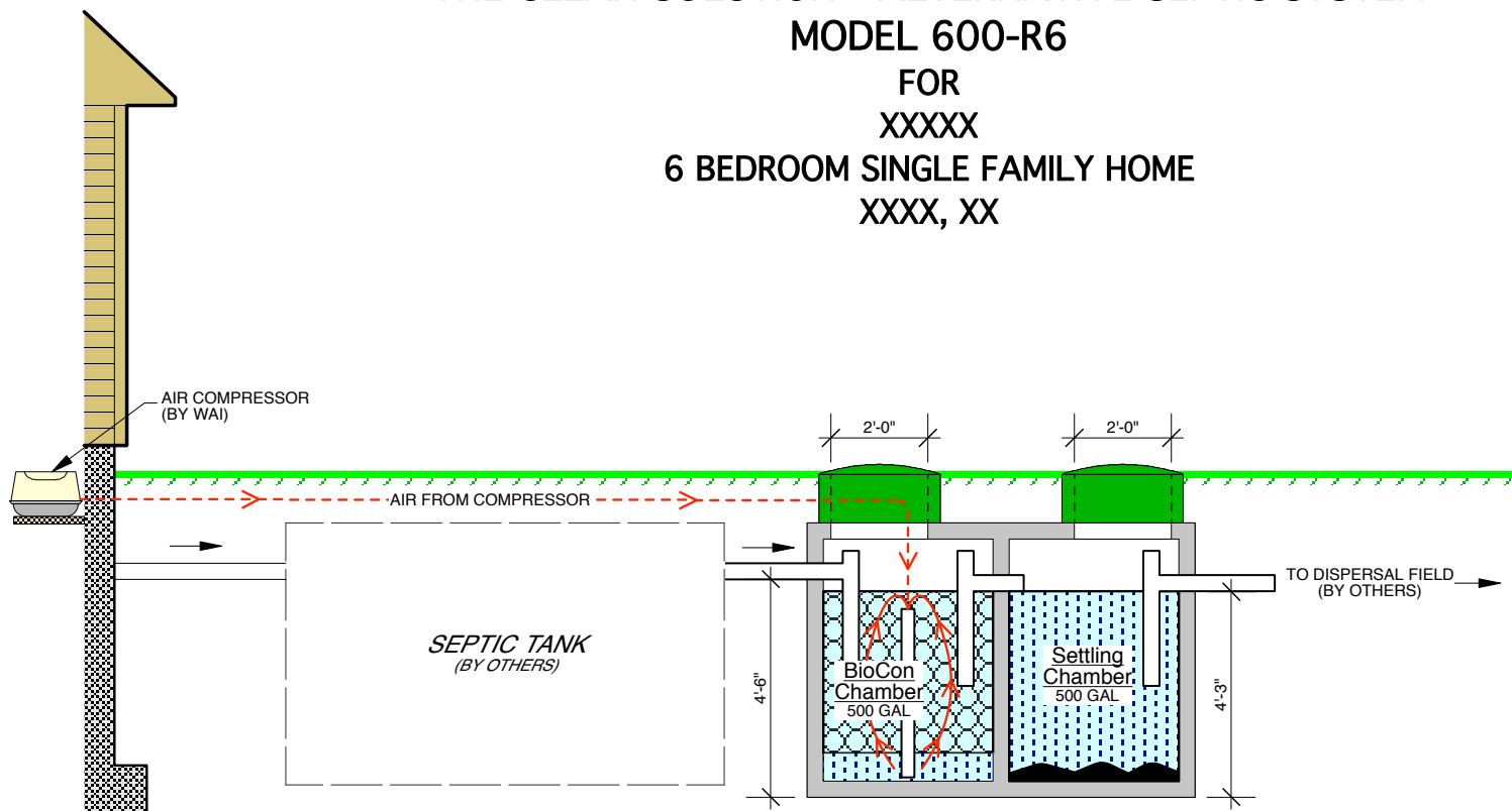
BioCon/Settling Tank 1,000 GAL 2 Compartment Tank (8'0"L x 5'4"W x 5'8"H)
