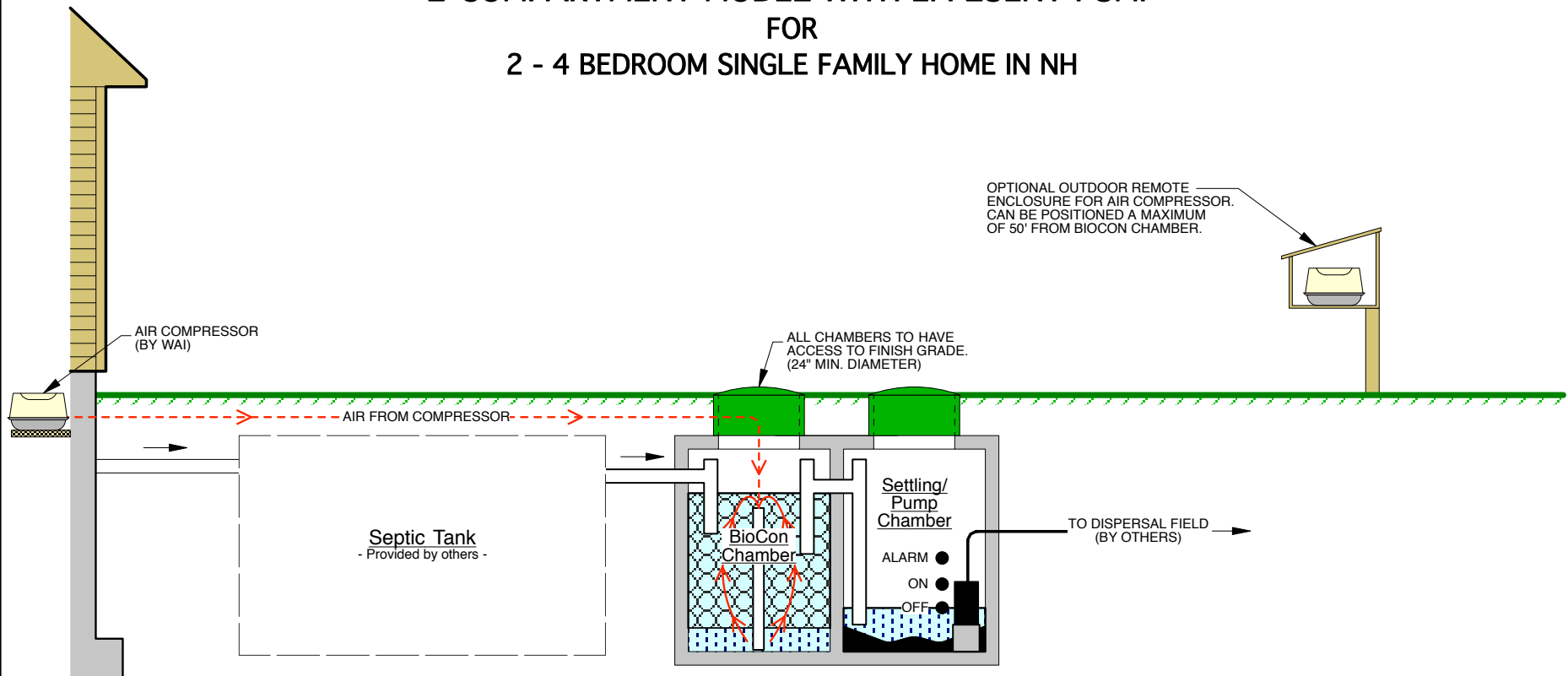
BioCon/Settling/Pump Tank 1,000-Gallon 2-Compartment (500/500 gal) Concrete Tank
